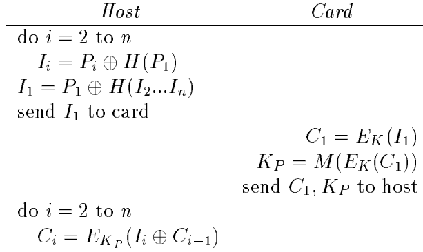
Figure 1: RKEP encryption of P to obtain C
