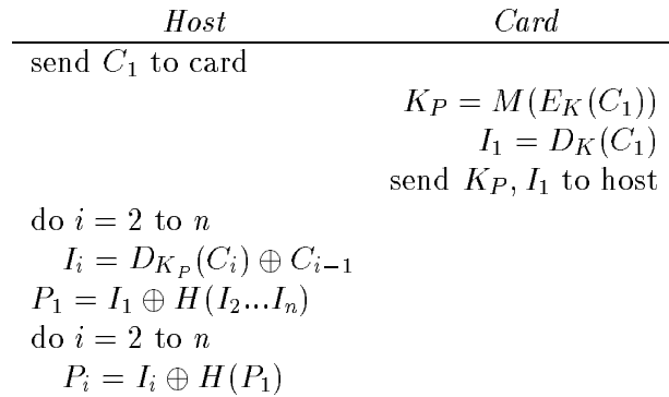
Figure 2: RKEP decryption of C to obtain P
